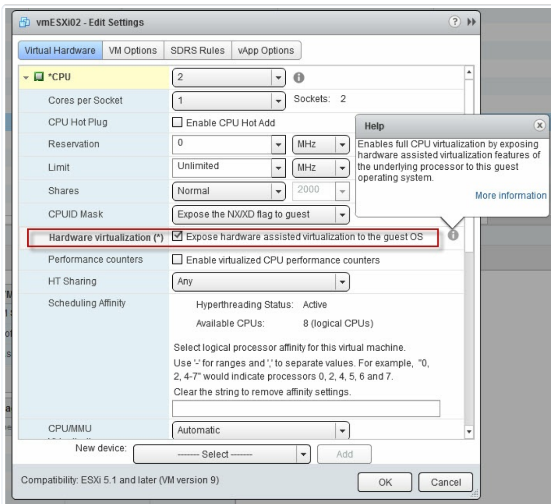
Hardware Virtualization field in the Edit Settings page
